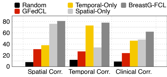
Fig. 6: Correlation between learned graph weights and clinical similarities. “Corr.” stands for “Correlation.”
