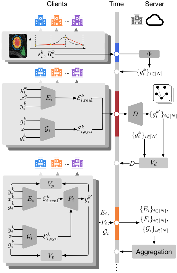
Fig. 3: Workflow of BreastG-FCL for Task k .
